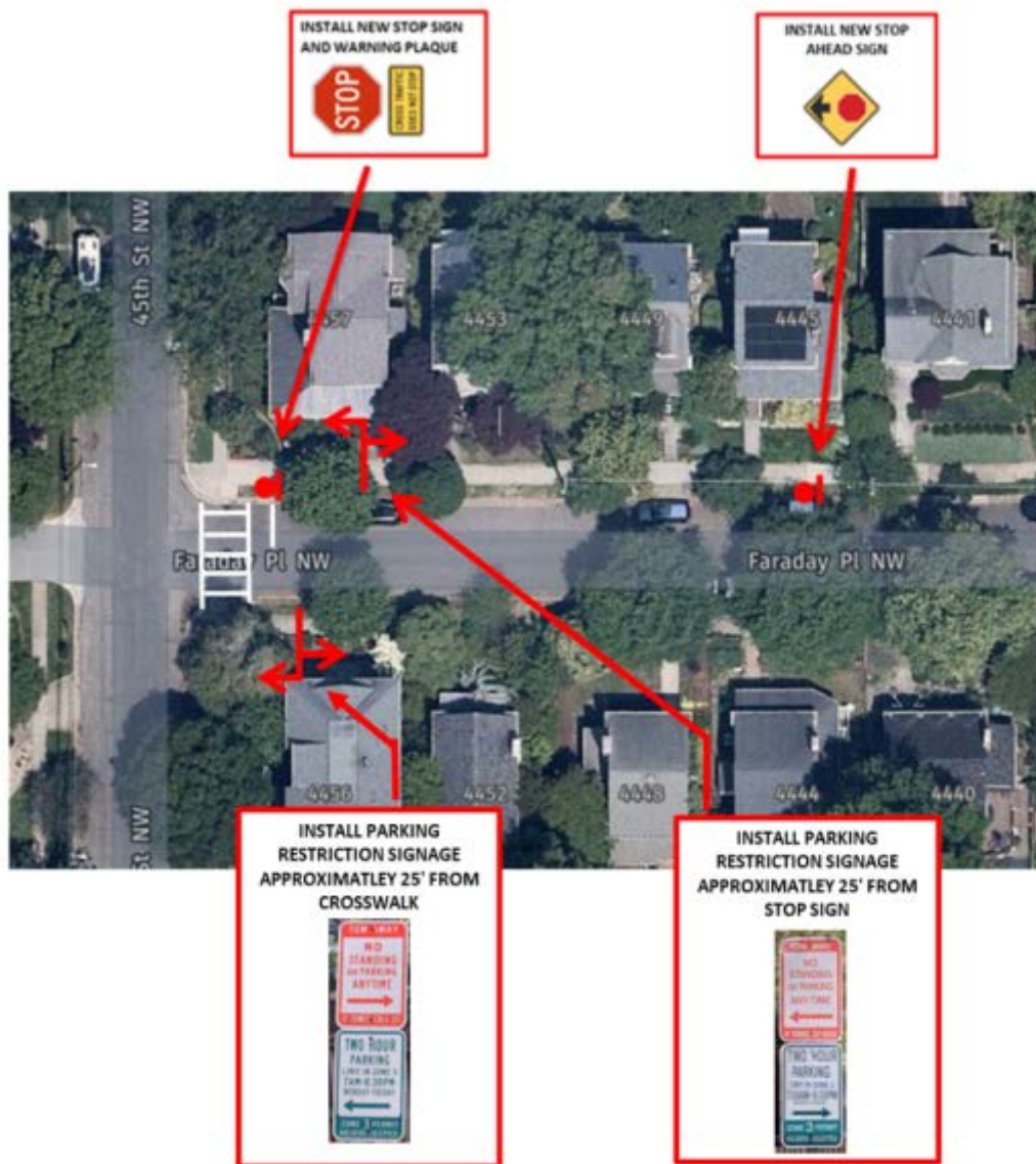
Figure 1: Proposed improvements for the “T” intersection of 45 th Street and Faraday Place, NW
