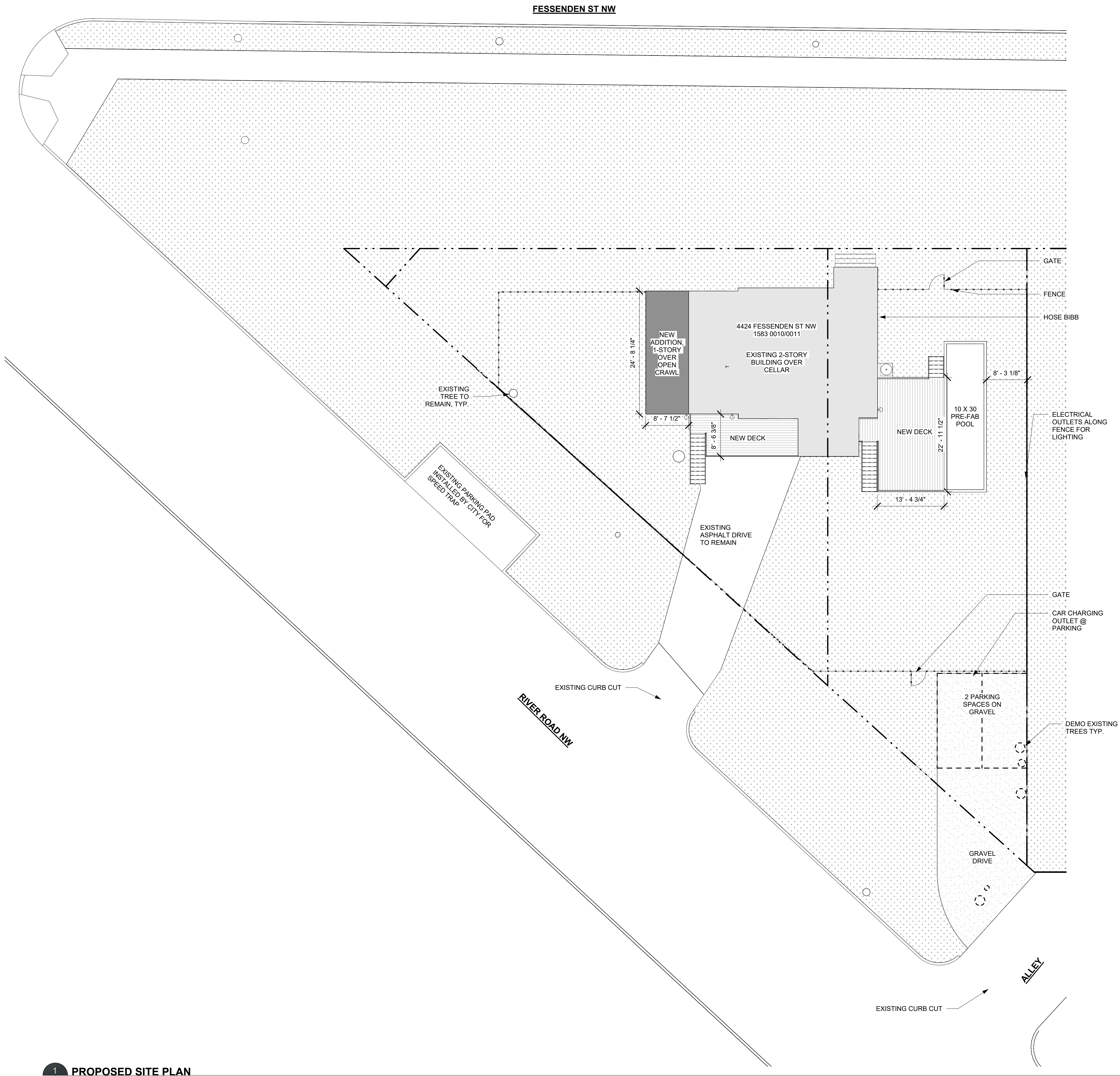
1 PROPOSED SITE PLAN A200 | C100 1" = 10'-0"
