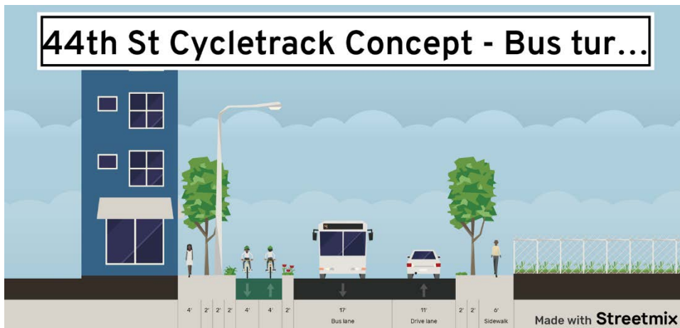
The cycletrack will be on the west side of 44 th in order to avoid conflicts with bus movements
