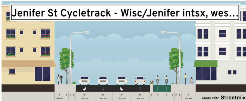
The cycletrack on the north side allows for the fewest conflicts with vehicles at the Wisconsin Ave intersection
